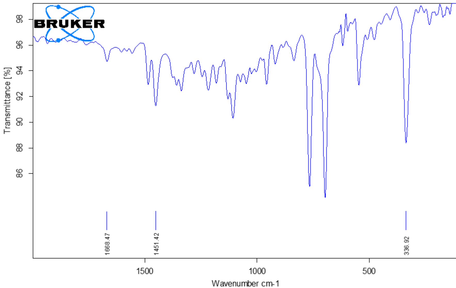
Figure S10. IR spectrum of trans -[PtCl 2 L 2 ] ( 1 )
