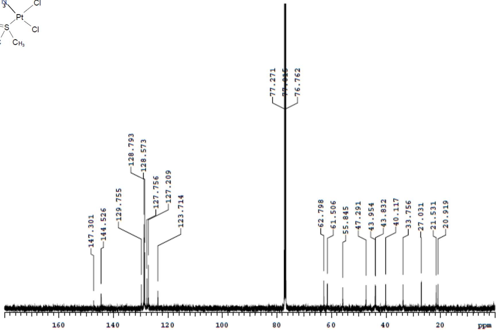
Figure S4b. ^{13}\text{C} NMR spectrum of the complex cis -[PtCl 2 (DMSO)L] ( 2 )
