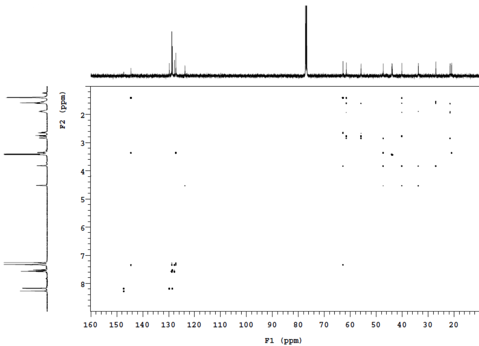
Figure S4d. ^1\text{H} - ^{13}\text{C} HMBC NMR spectrum of the complex cis -[PtCl 2 (DMSO)L] ( 2 )
