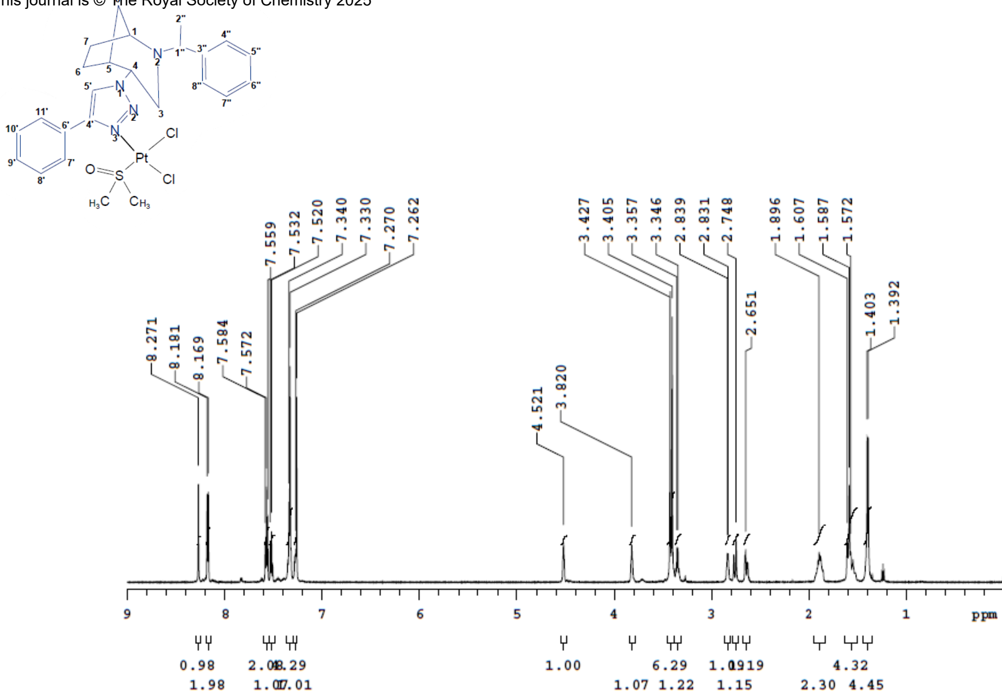
Figure S4a. 1 H NMR spectrum of the complex cis -[PtCl 2 (DMSO)L] (2)
