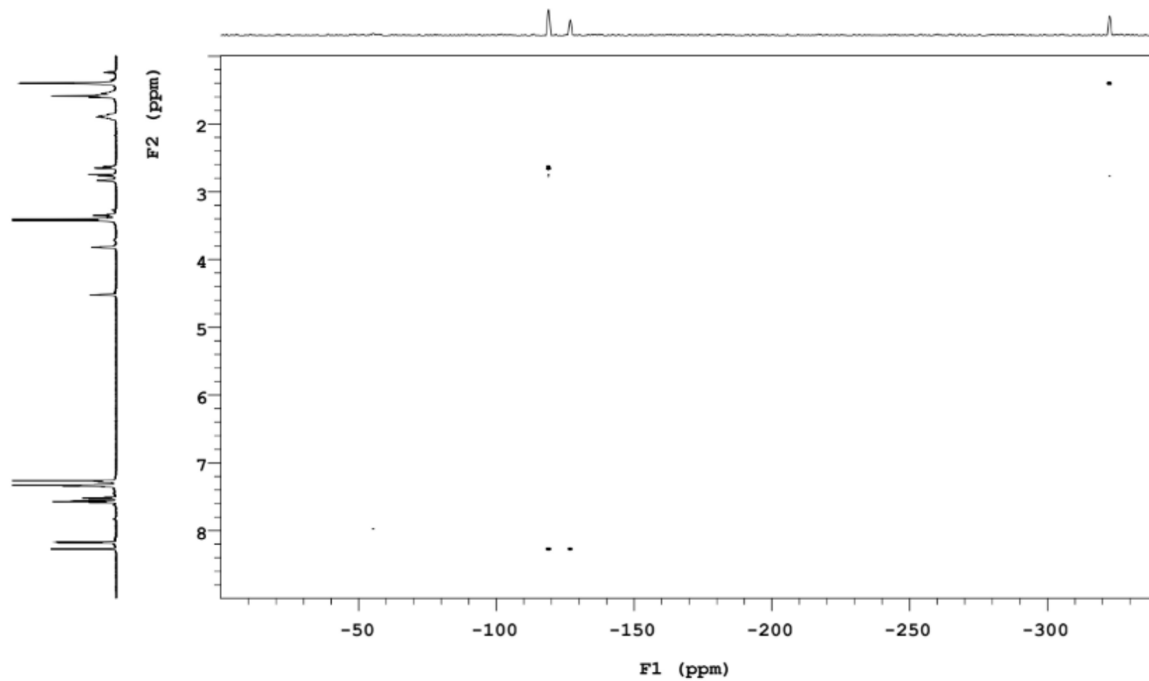
Figure S4e. ^1\text{H} - ^{15}\text{N} HMBC NMR spectrum of the complex cis -[PtCl 2 (DMSO)L] ( 2 )
