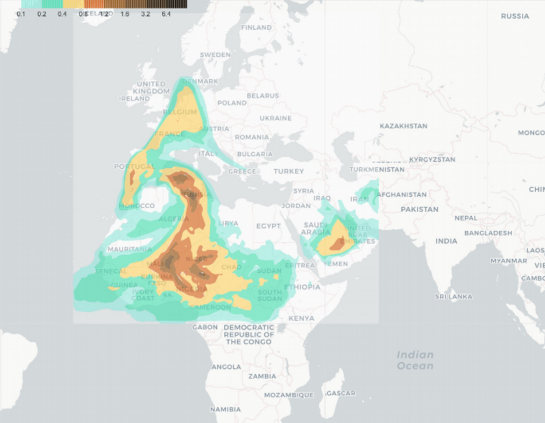
MULTI-MODEL Dust Optical Depth (550nm) Valid: 00h 19 Mar 2022 (H+12)
