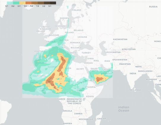
MULTI-MODEL Dust Optical Depth (550nm) Valid: 00h 18 Mar 2022 (H+12)
