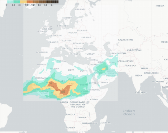
MULTI-MODEL Dust Optical Depth (550nm) Valid: 00h 16 Mar 2022 (H+12)
