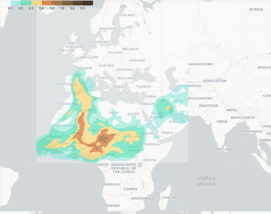
MULTI-MODEL Dust Optical Depth (550nm) Valid: 00h 17 Mar 2022 (H+12)
