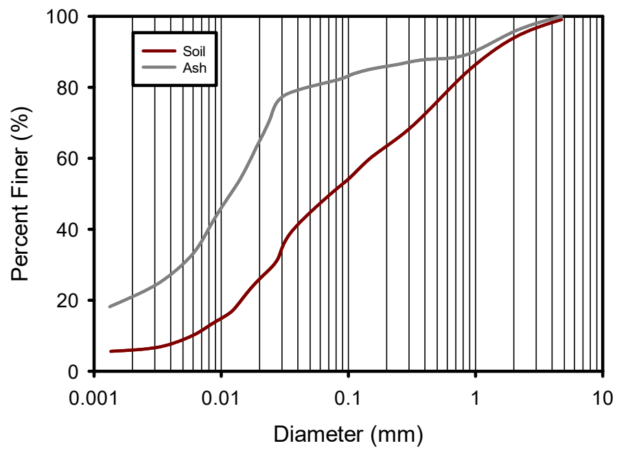
SI Figure 1. Particle size distribution curves of soil and ash sampled from the study site.
