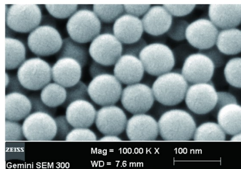
Supplementary data. Fig. 1 Electron microscope image of PS-NPs.
