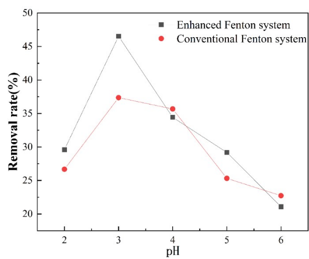
Fig. S1 Influence of pH on COD removal rate
