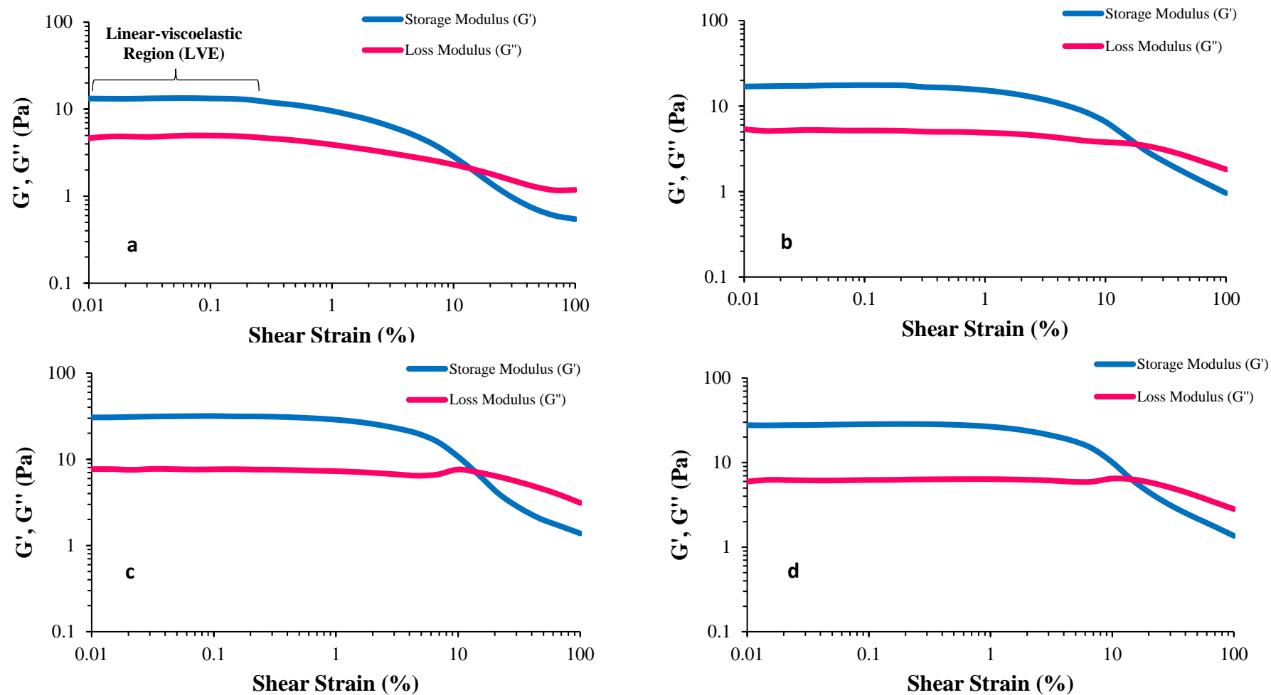
Fig. S1 Viscoelastic curves of samples subjected to (a) conventional homogenization, (b) US for 1 min, (c) US for 3 min and (d) US for 5 min
