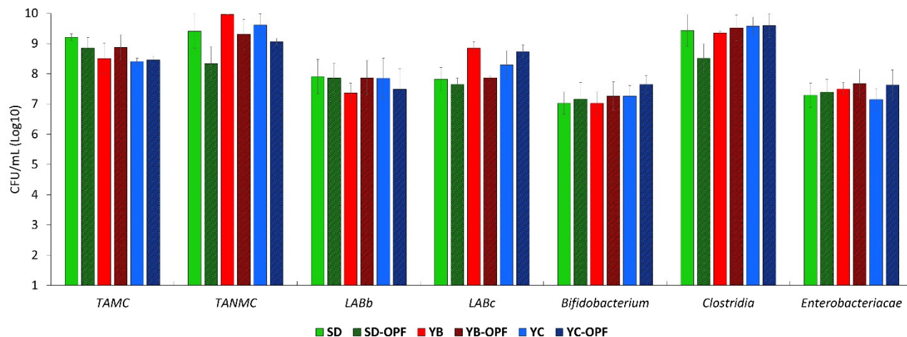
Supplementary Figure S1: Viable bacterial count (Log 10 CFU/mL ± SD) of faecal microbiota observed in batches simulating the colonic fermentation of permeate in vitro . Permeate solution contained the residual from the simulated digestion of muffin differing for the addition of OPF and type of fermentation (with chemical yeast, YC; baker's yeast YB; or type-II sourdough, SD). Abbreviations: TAMC, total aerobic microbial count; TANMC, total anaerobic microbial count; LABb, bacillus-shaped lactic acid bacteria; LABc, coccus-shaped lactic acid bacteria.
