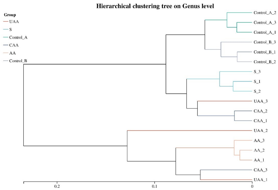
Figure S2 Hierarchical clustering tree on genus level
