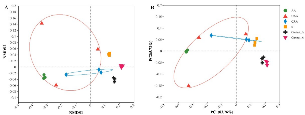
Figure S1 (A) NMDS; (B)PCoA
