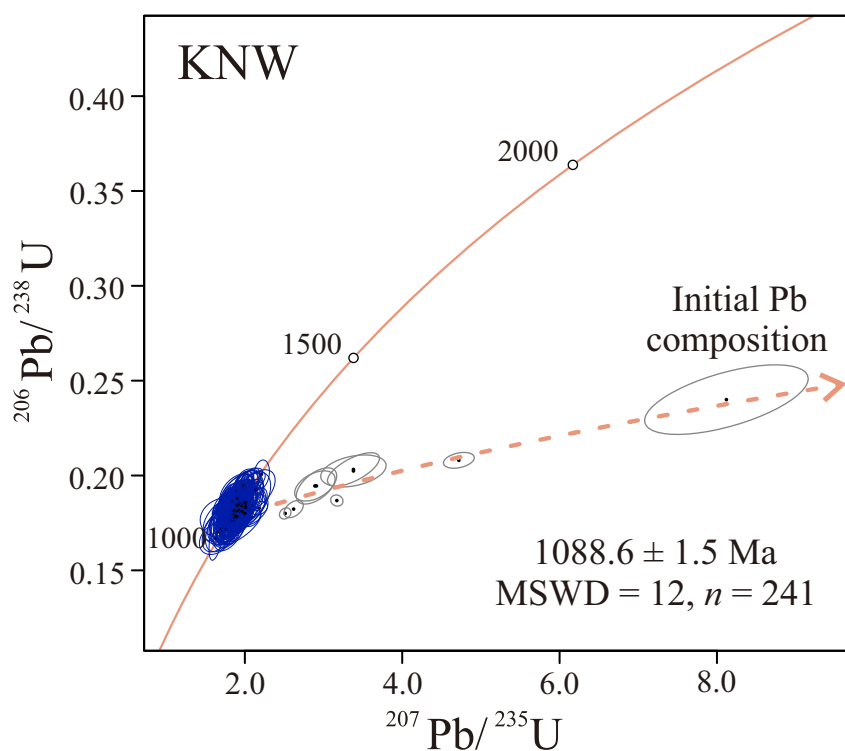
ESI Figure S2. Concordia diagram of U–Pb ages obtained using LA–ICP–MS. KNW rutile contains very low common Pb with only 12 of 241 spot analyses show amount of common Pb ( f_{206} : 0–20%)
