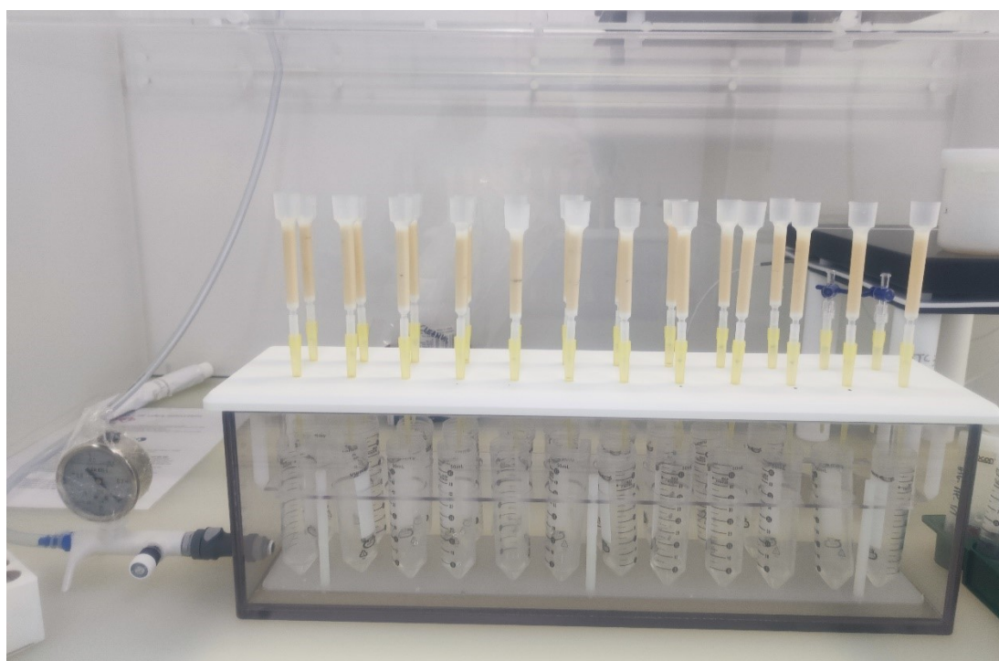
Figure S1 Vacuum box used for the chromatographic isolation procedure.
