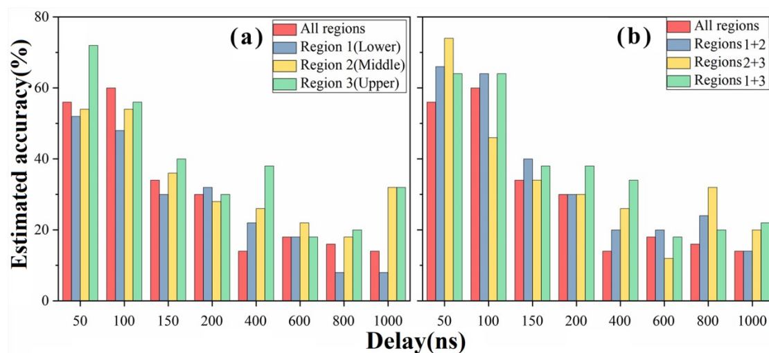
Evaluation accuracy of aging grade models based on plasma RSD image from different regions (4 shots RSD).
