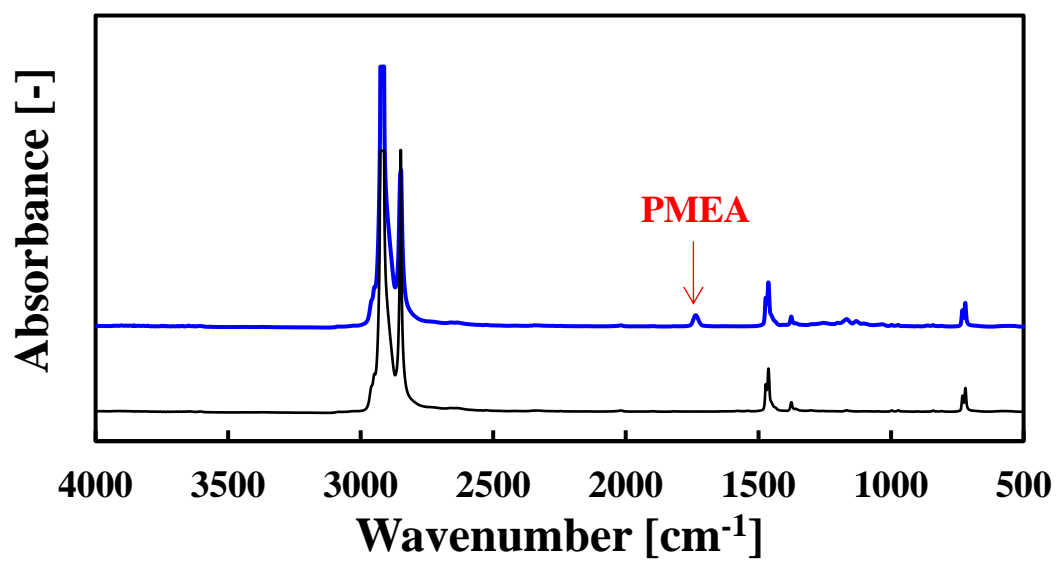
Figure S1. FT-IR spectra of unmodified (black) and modified membranes with a grafting amount of 0.12 mg cm -2 (blue), which were analyzed by the transmission method.
