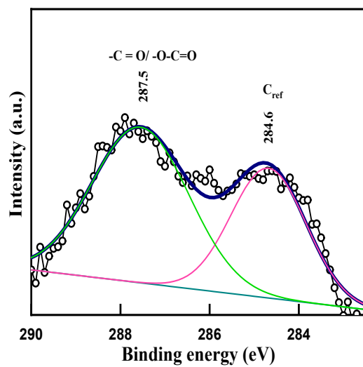
Fig. S4 C1s XPS spectrum of 2.
