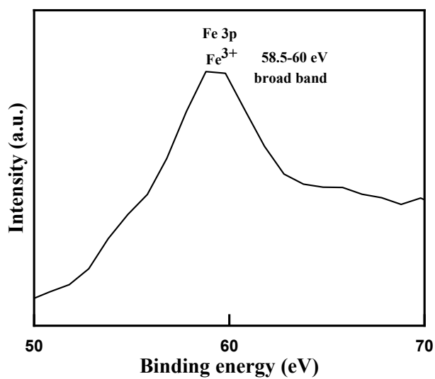
Fig. S5 Fe 3p XPS spectrum of 2.
