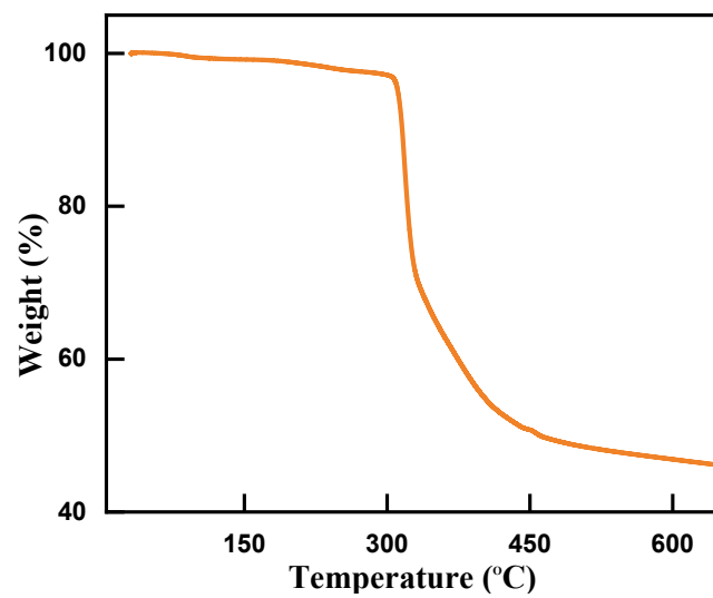
Fig. S1 Thermogravimetric Analysis of 2 .
