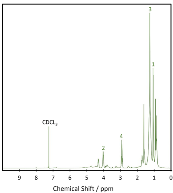
Fig. S2 1 H NMR spectrum for P45
