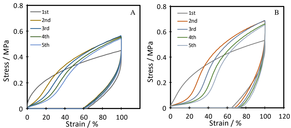
Fig. S3 Cyclic tensile plots for P40 carried out at (A) 100 mm.min -1 and (B) 200 mm.min -1 , with no rest time given between cycles.
