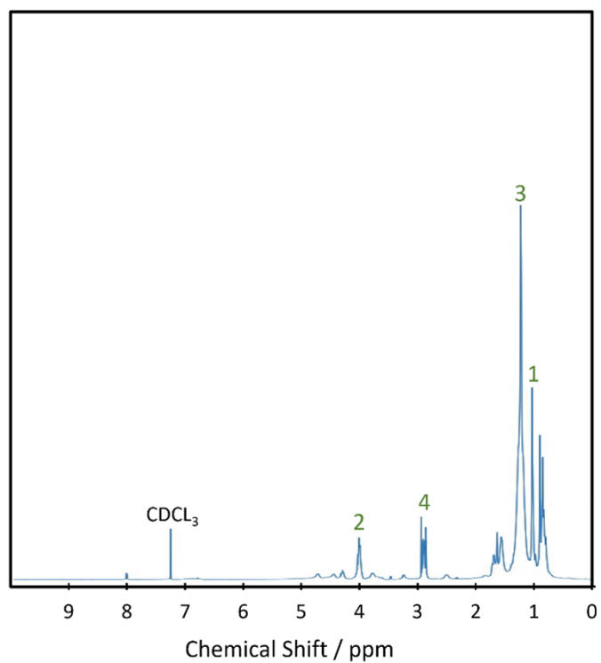
Fig. S1 1 H NMR spectrum for P35
