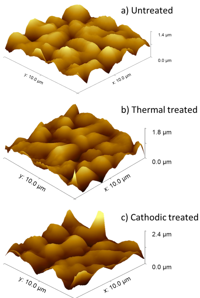
Fig.S.I. 1: 3D topographies of the samples: a) Untreated, b) Thermal treated, and c) Cathodic treated. Obtained by AFM in intermittent mode.
