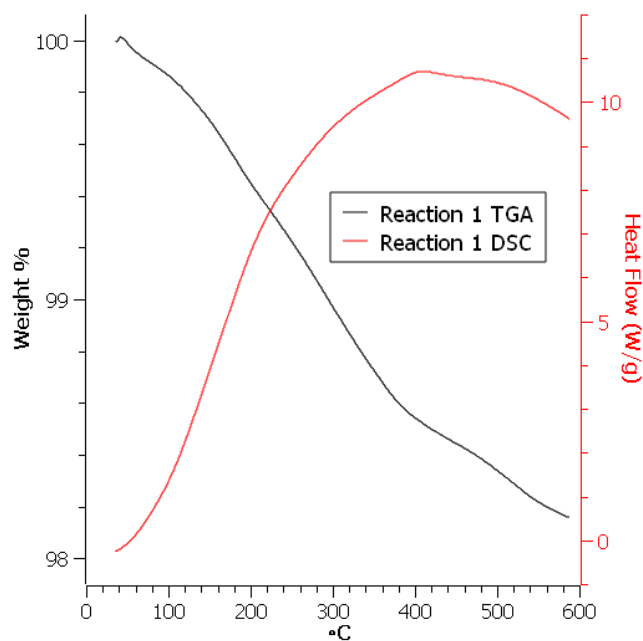
Fig. S3 TGA-DSC of the results of reaction 1.
