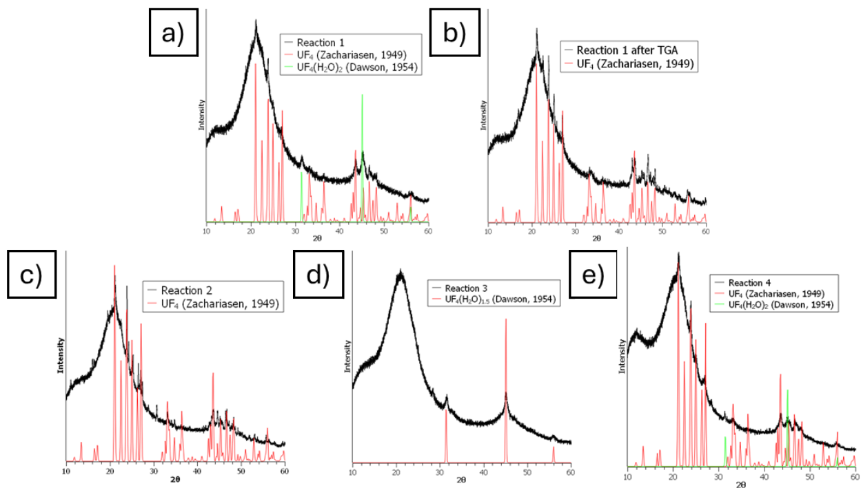
Fig. S2 XRD patterns resulting from a) reaction 1, b) reaction 1 after TGA-DSC, c) reaction 2, d) reaction 3, and e) reaction 4.
