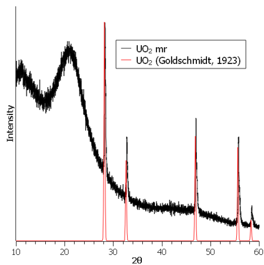
Fig. S1 PXRD of the UO 2 mr starting material.
