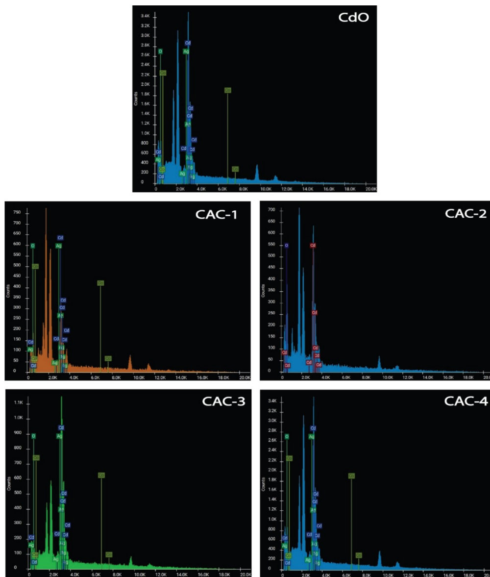
Figure 1: EDS graph of pure CdO and the Ag-Co dual-doped CdO thin films.
