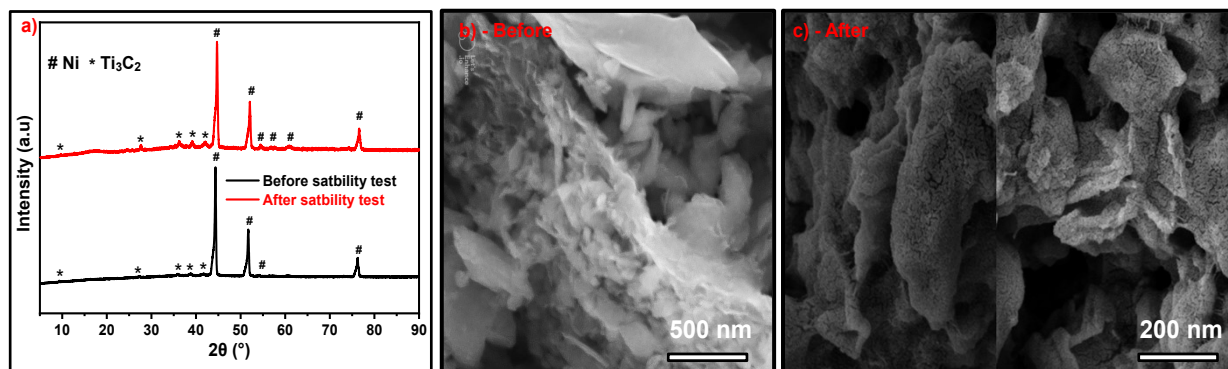
Figure S1:- a) XRD of Post stability test [b) SEM images of before and after stability test of the MMXene catalyst in 2 M NaOH
