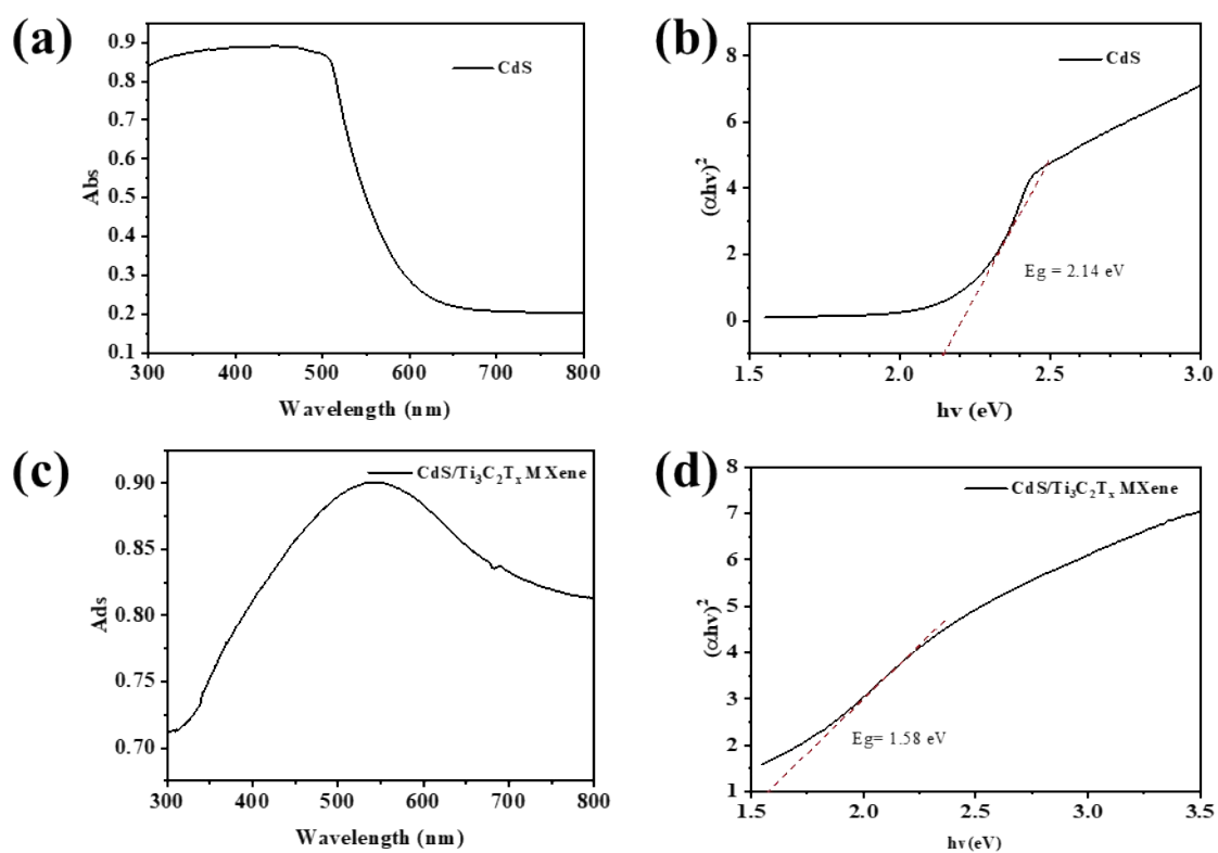
Figure S1. UV-Vis DRS (a, c) and Tauc plots (b, d) of CdS and CT2 heterostructure, respectively.
