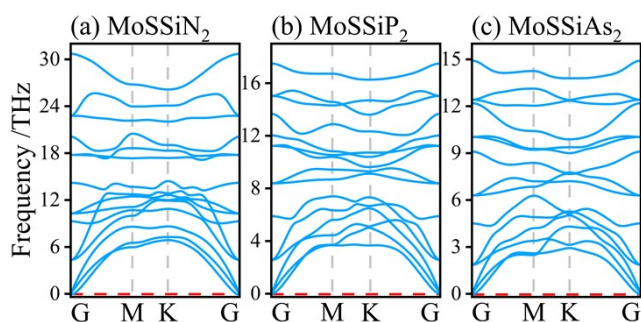
Fig. S1. The phonon dispersion curve after applying a 4% compressive strain of Janus MoSSiX 2 (X=N, P, As) monolayers.
