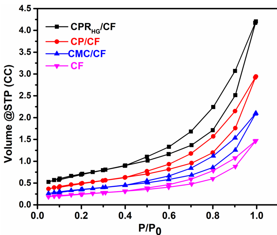
Fig.S2: N 2 adsorption-desorption curves for the CPR HG /CF and its counterparts
