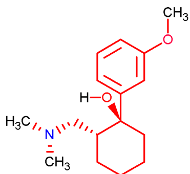
Fig. S1: Chemical structure of tramadol
