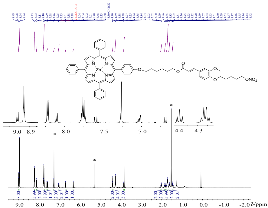
Figure 1.12. 1 H NMR of compound 7e
