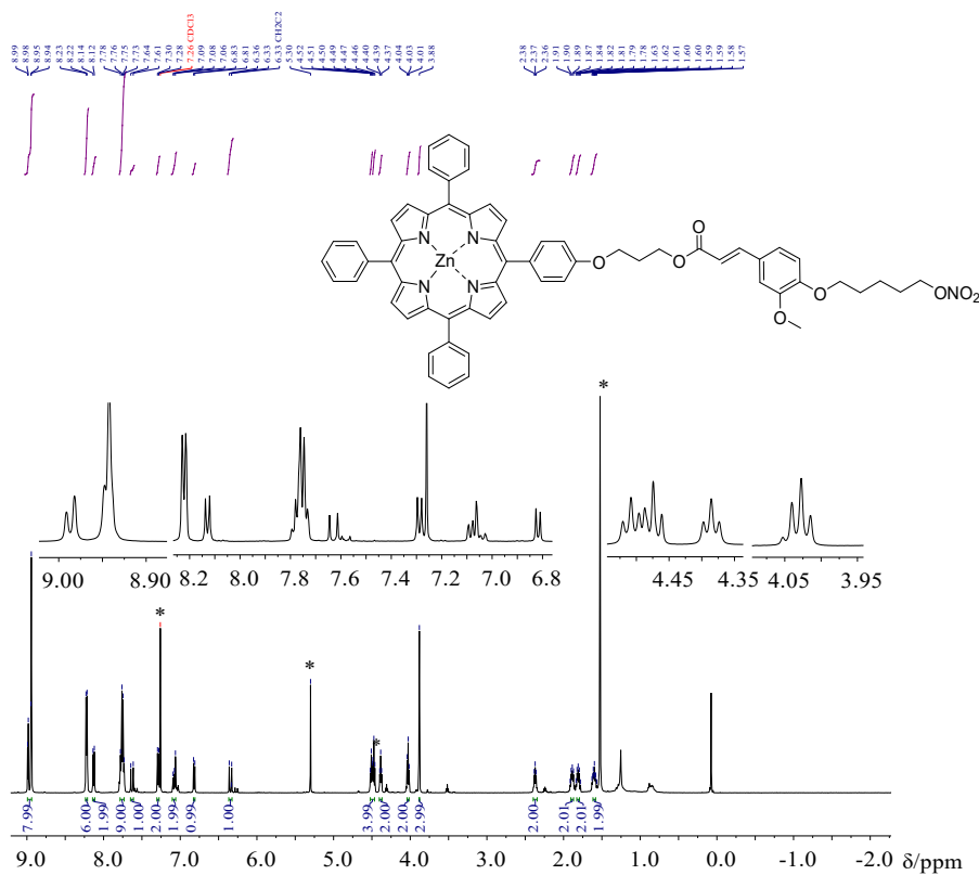
Figure 1.9. 1 H NMR of compound 7b
