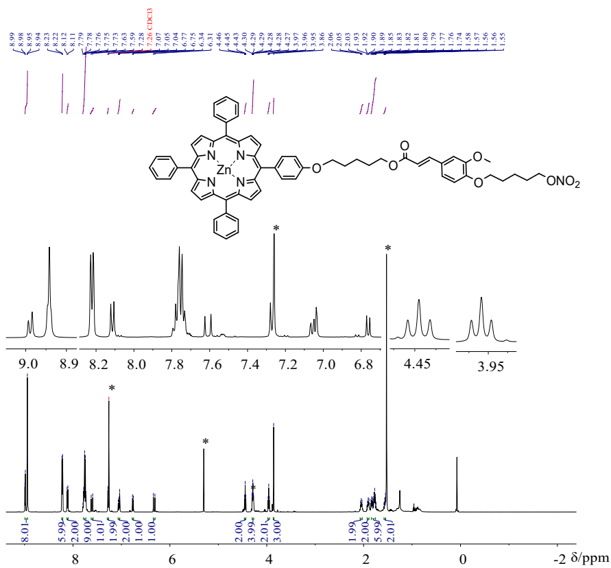
Figure 1.10. ^1\text{H} NMR of compound 7c
