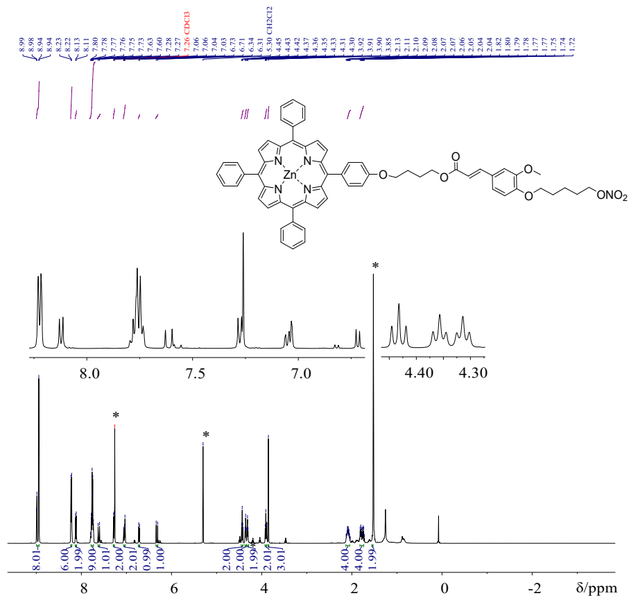
Figure 1.10. ^1\text{H} NMR of compound 7c
