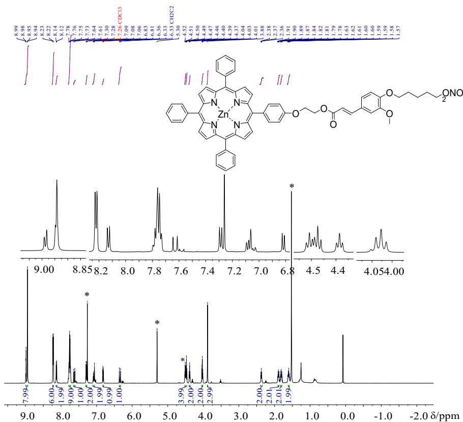
Figure 1.8. 1 H NMR of compound 7a
