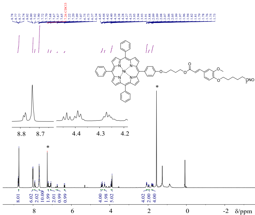
Figure 1.15. 1 H NMR of compound 8c
