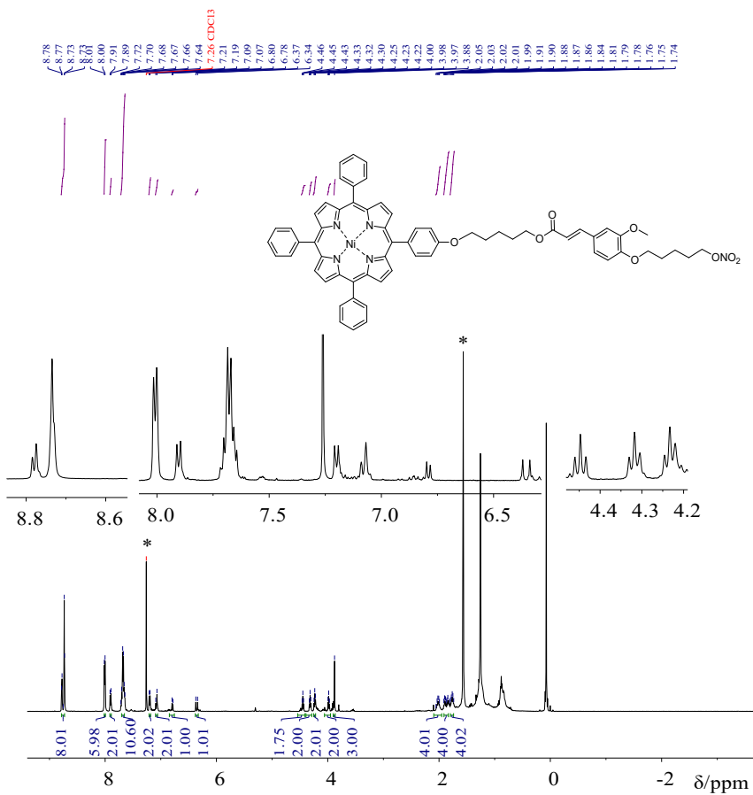
Figure 1.16. 1 H NMR of compound 8d
