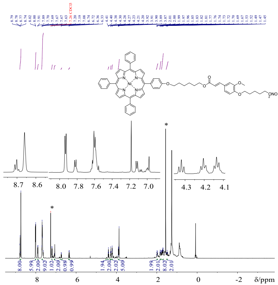
Figure 1.17. 1 H NMR of compound 8e
