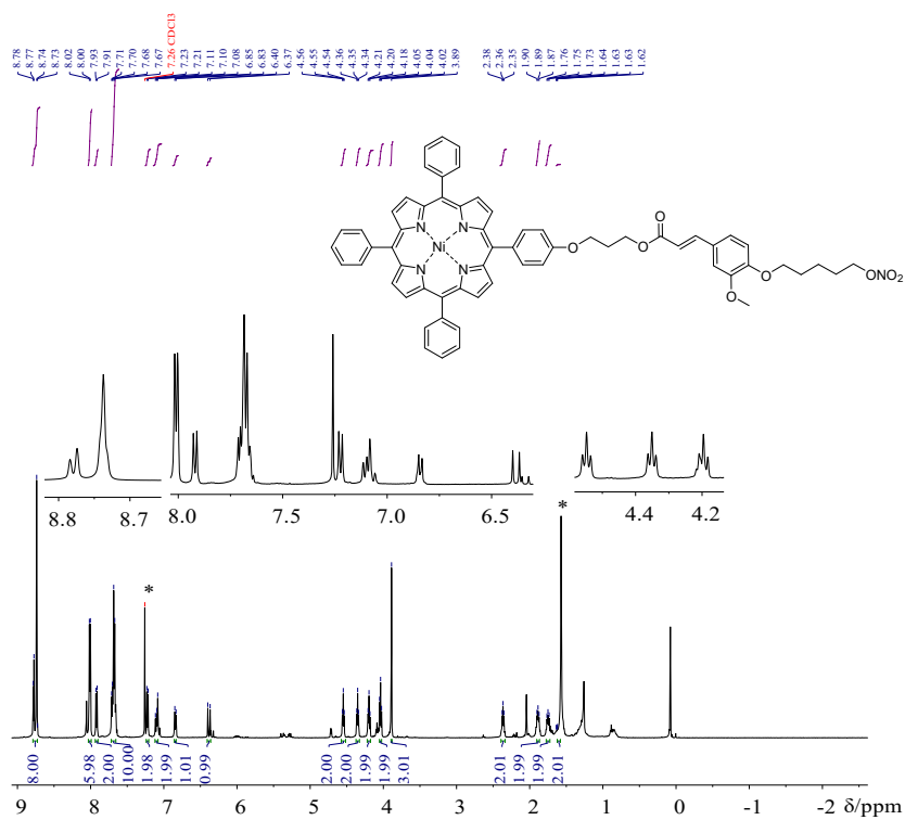
Figure 1.13. 1 H NMR of compound 8a
