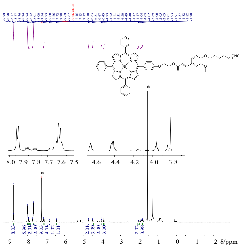
Figure 1.13. 1 H NMR of compound 8a
