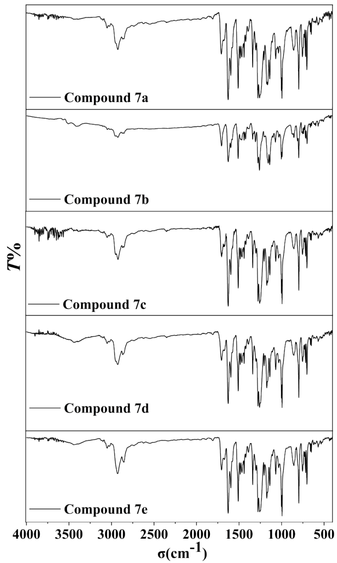
Figure 4.2. Infrared spectra of compounds 7a-7e
