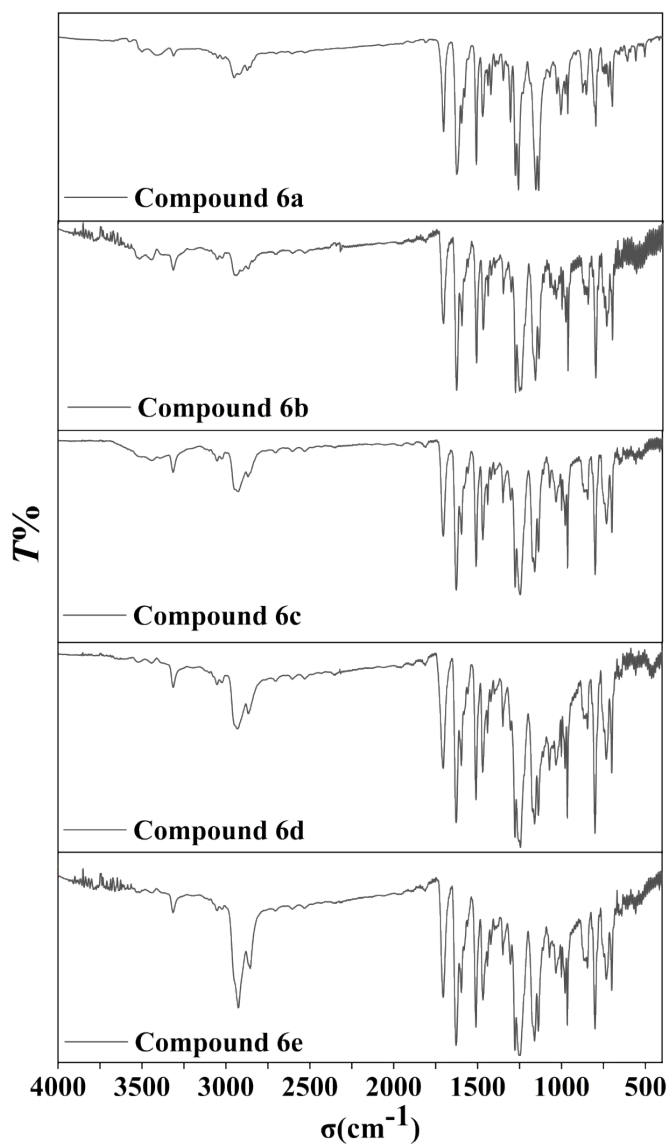
Figure 4.1. Infrared spectra of compounds 6a-6e
