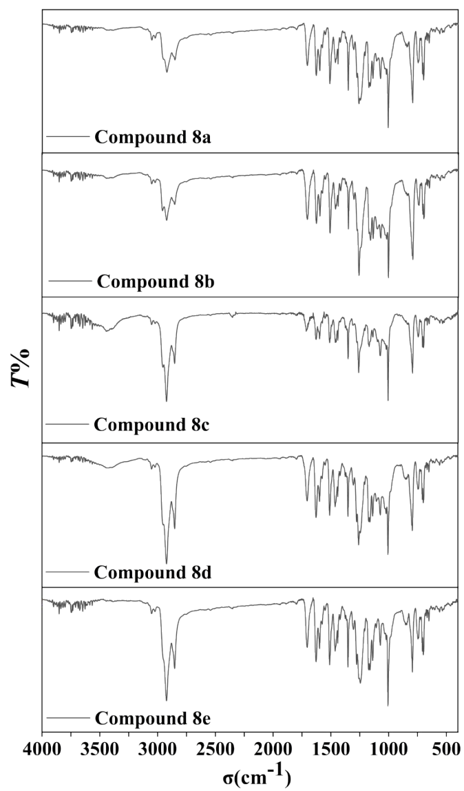
Figure 4.3. Infrared spectra of compounds 8a-8e
