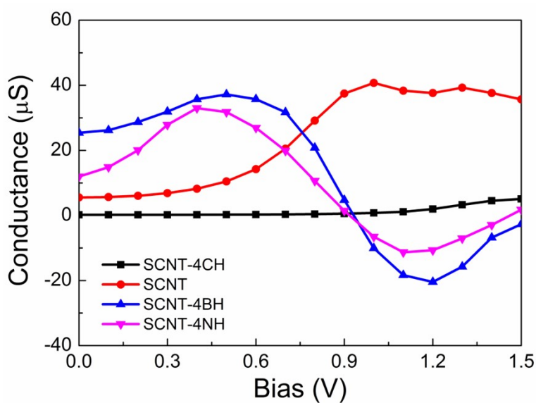
Figure S1. The conductance characteristics of SCNT-4CH, SCNT, SCNT-4BH and SCNT-4NH junctions.
