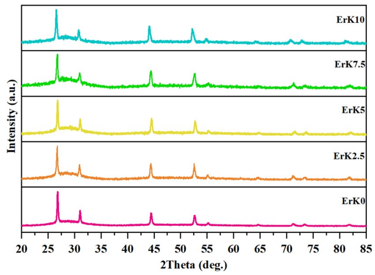
Figure S1. XRD pattern of \beta -PbF 2 :Er 3+ /K + GCs varying with K + concentration.
