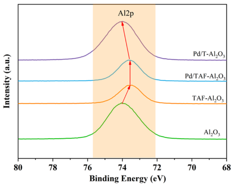
Fig. S1 XPS of different samples with Al
