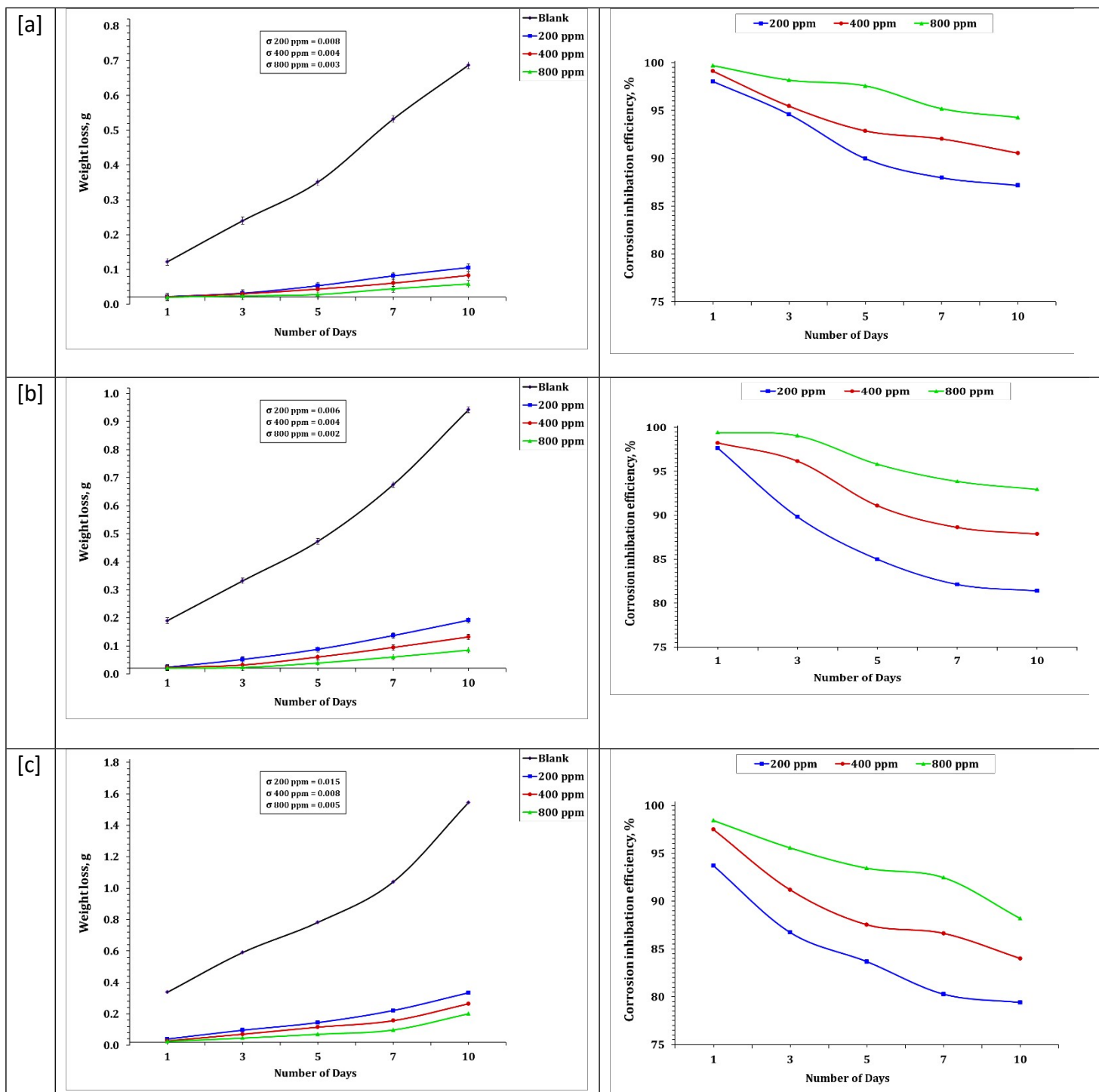
Figure S1: Variation in weight loss of carbon steel coupons (left side) and corrosion inhibition (right side) versus the testing time; [a] in pure water, [b] in formation water, [c] in diesel fuel and [d] in sulfuric acid.
