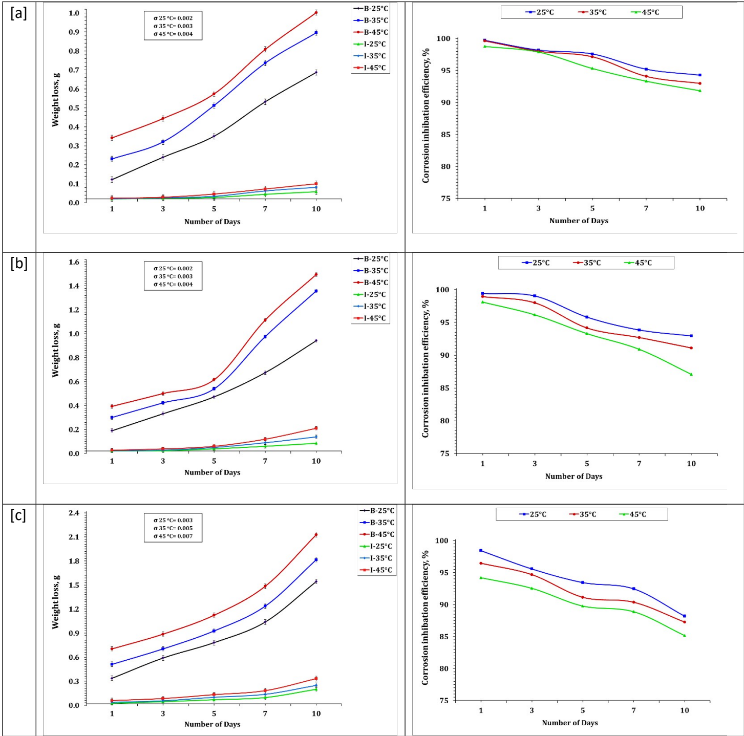
Figure S2: Variation in weight loss of carbon steel coupons (left side) and corrosion inhibition (right side) versus the testing time at different temperature; [a] in pure water, [b] in formation water, [c] in diesel fuel and [d] in sulfuric acid.
