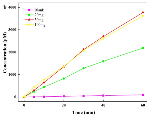
Fig. S6 Photocatalytic H_2O_2 production with different masses of Pd/3PEI/BOC.
