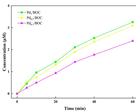
Fig. S2 Photocatalytic activity for Pd 0.1 /BOC, Pd 0.5 /BOC and Pd 1.0 /BOC.
