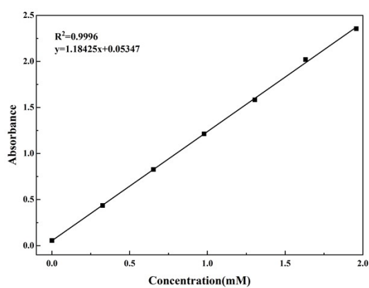
Fig. S5 The linear fitting formula of standard H_2O_2 concentration.
