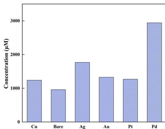
Fig. S4 Photocatalytic activity of metal species (0.5 wt%) loaded on BiOCl.
