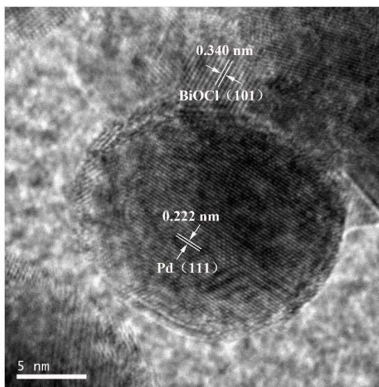
Fig. S3 HRTEM image of Pd/BOC.
