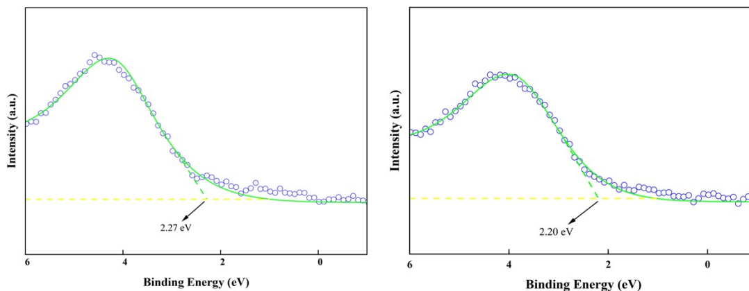
Fig. S1 Valence-band XPS spectra of Pd/BOC and Pd/3PEI/BOC.
