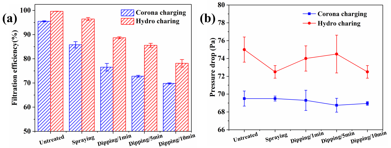
Fig. S2 The effects of ethanol spraying and impregnation treatment on the filtration performance of electret melt blown samples: (a) filtration efficiency, (b) filtration resistance
