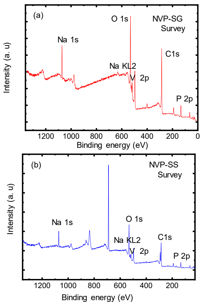
Fig. S1. XPS survey spectrum recorded for the NVP-SG and NVP-SS samples.
