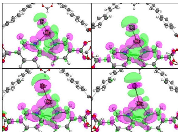
Fig. S1 Illustration of the electron density difference (EDD) (isovalue = 0.001 e a.u. -3 ) of the CuX-deposited UiO-67(bpy) MOF (X = F, Cl, Br, and I). Green and pink regions represent the areas of electron accumulation and electron depletion, respectively.
