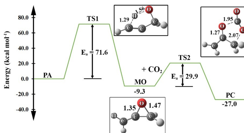
Fig. S2 Energetic profile for the carboxylative cycloaddition of CO 2 with propargyl alcohol through the formation of methyleneoxirane (MO) without a catalyst.
