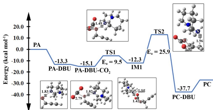
Fig. S3 Energetic profile for the carboxylative cycloaddition of CO 2 with propargyl alcohol catalyzed by the DBU base.
