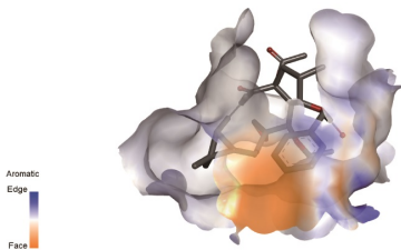
(c) Aromatic interactions between euphobiasteroid and HSP90AA1
