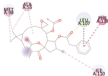
(b) 2D interaction plane diagram of euphobiasteroid with HSP90AA1
