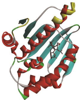
(a) 3D interaction structure of euphobiasteroid with HSP90AA1
