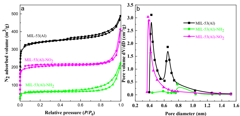
Figure S1 Nitrogen adsorption-desorption isotherms and corresponding pore size distributions of MIL-53(Al), MIL-53(Al)-NO 2 and MIL-53(Al)-NH 2
