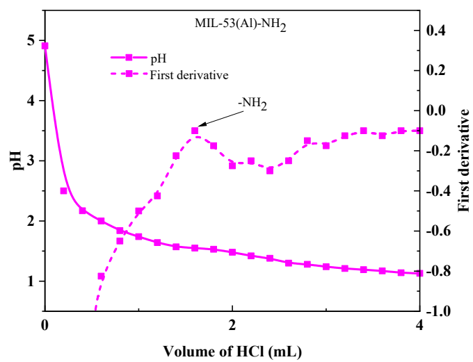
Figure S5 Titration and derivative curve of MIL-53(Al)-NH 2 with HCl (0.1M)
