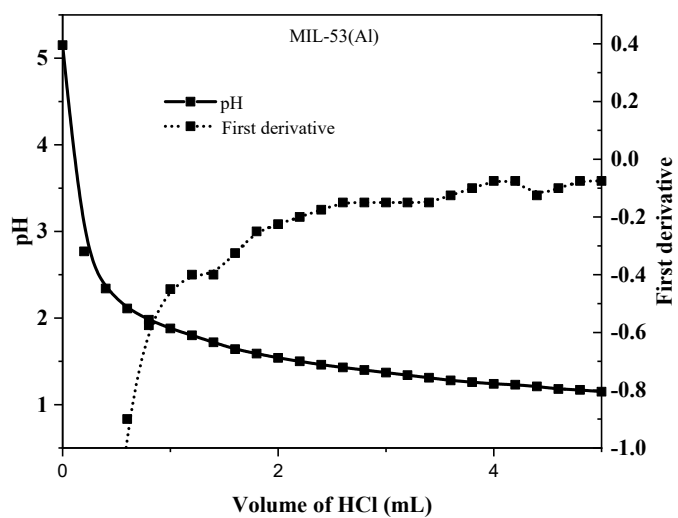
Figure S3 Titration and derivative curve of MIL-53(Al) with HCl (0.1M)
