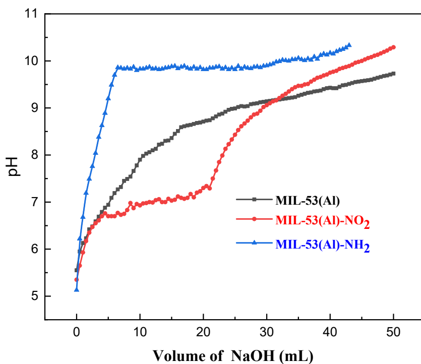
Figure S2 Titration and derivative curve of MIL-53(Al), MIL-53(Al)-NO 2 and MIL-53(Al)-NH 2 with NaOH (0.005M)
