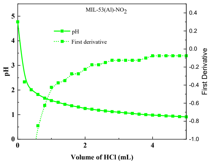
Figure S4 Titration and derivative curve of MIL-53(Al)-NO 2 with HCl (0.1M)
