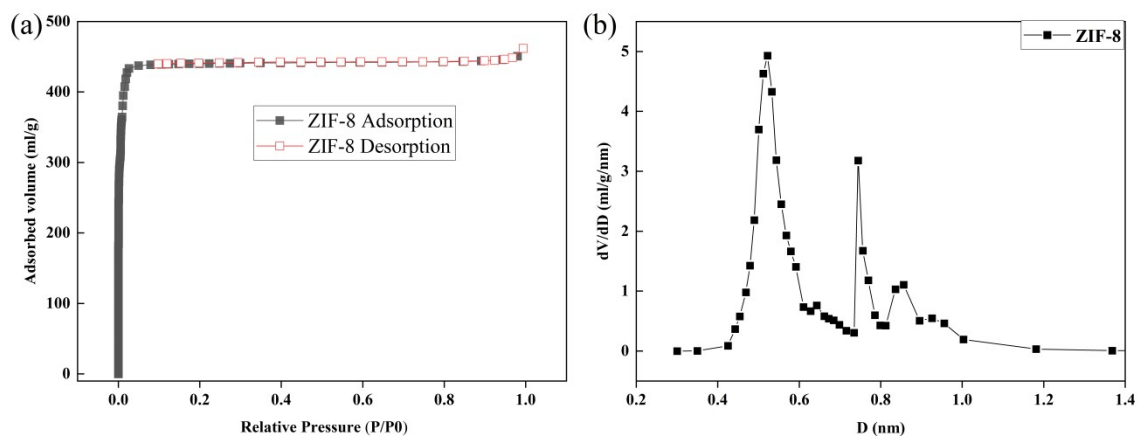
Fig. S1. shows this. (a) N_2 adsorption/desorption isotherms of ZIF-8 and (b) pore size distributions of ZIF-8.
