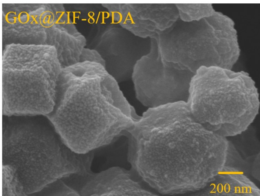
Fig. S3. SEM image of GOx@ZIF-8/PDA after three times of reuse.
