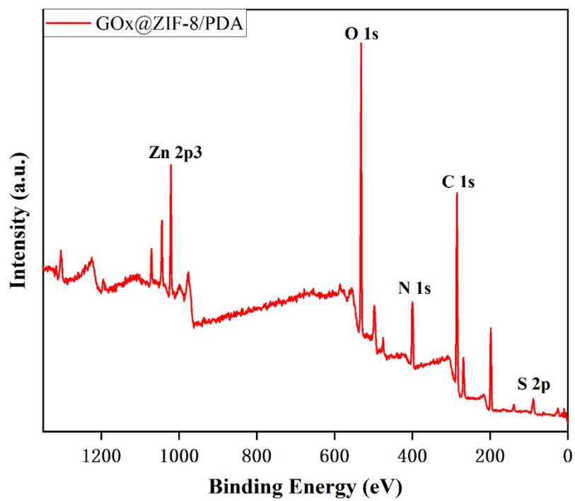
Fig. S2. General XPS drawing for GOx@ZIF-8/PDA
