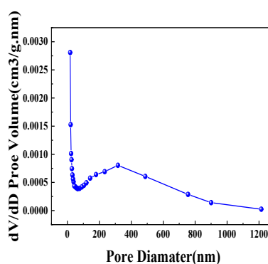
Fig. S1 Pore size distribution graph of N-TFACOP
