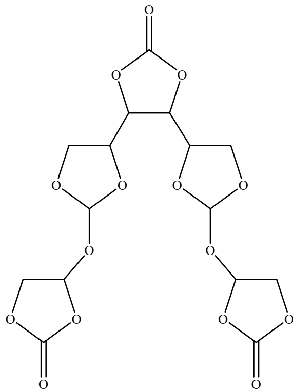
Figure S2. The structure reported in Ota's study.
