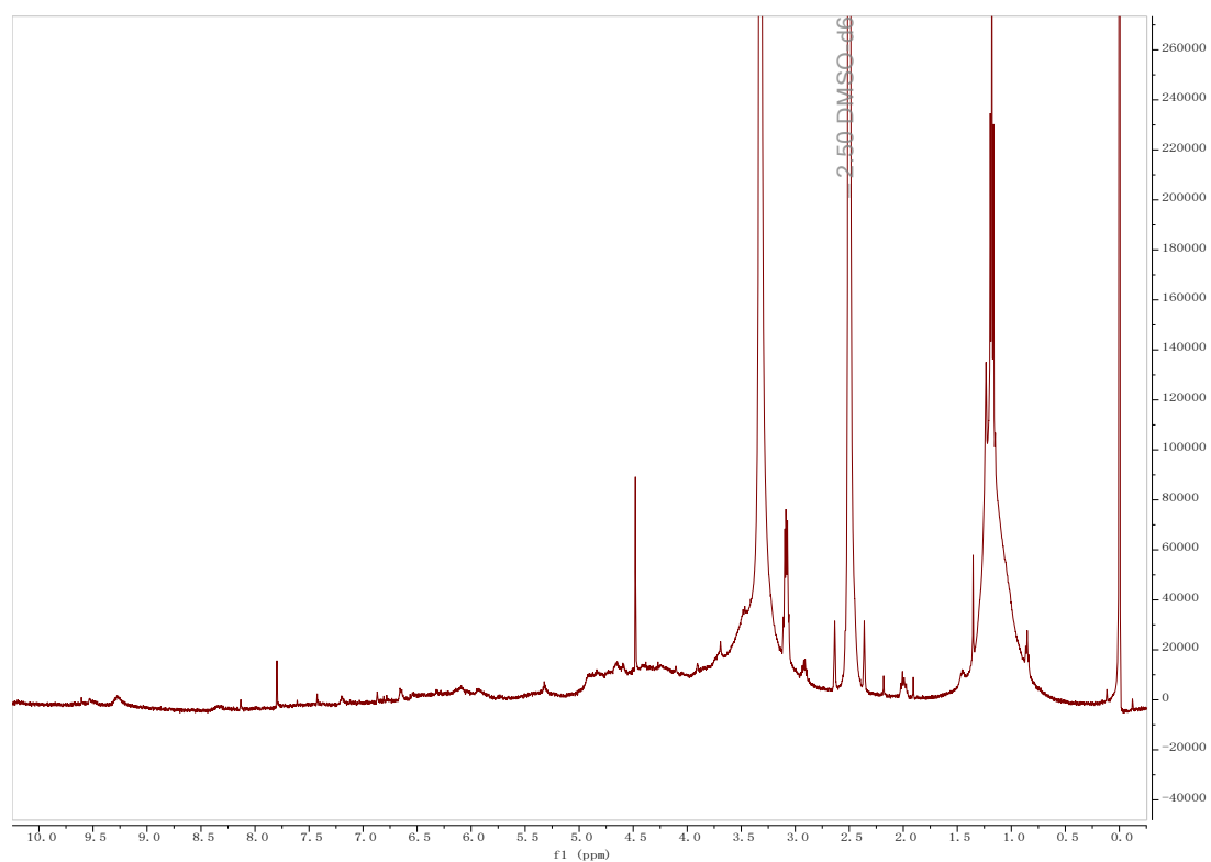
Figure S1. 1 H NMR spectrum of polyVC Sys (measured at 25 °C).
