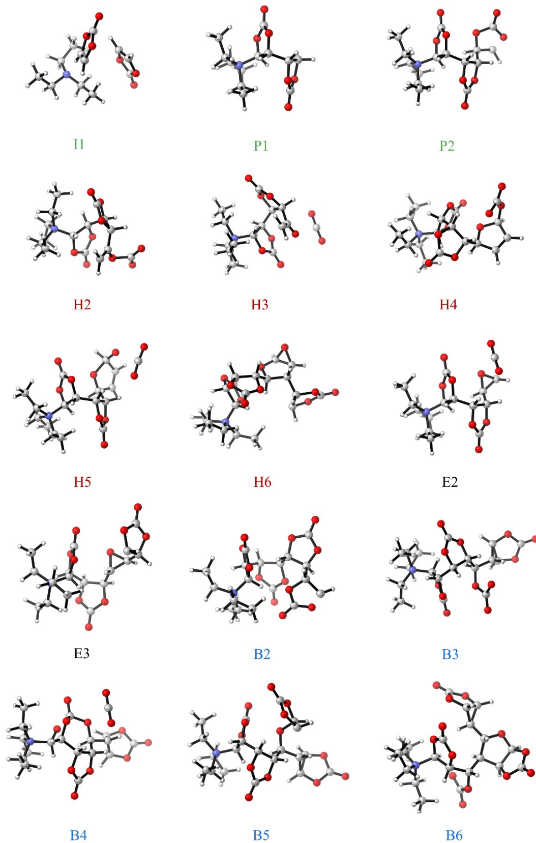
Figure S3. Structures of intermediates and minima.
