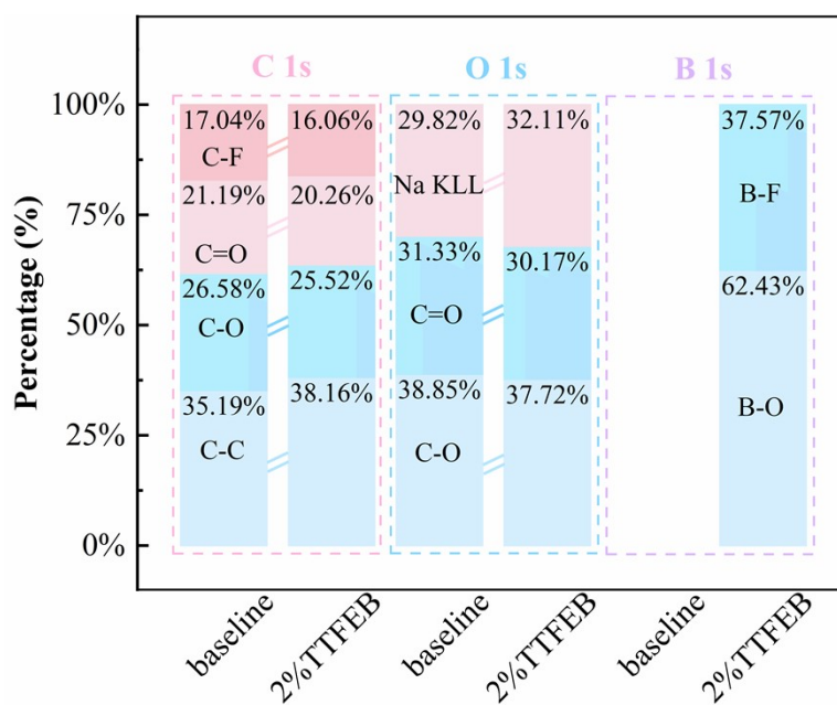
Fig. S2. The detailed percentage of each component from C1s, O1s, and B1s XPS spectra.
