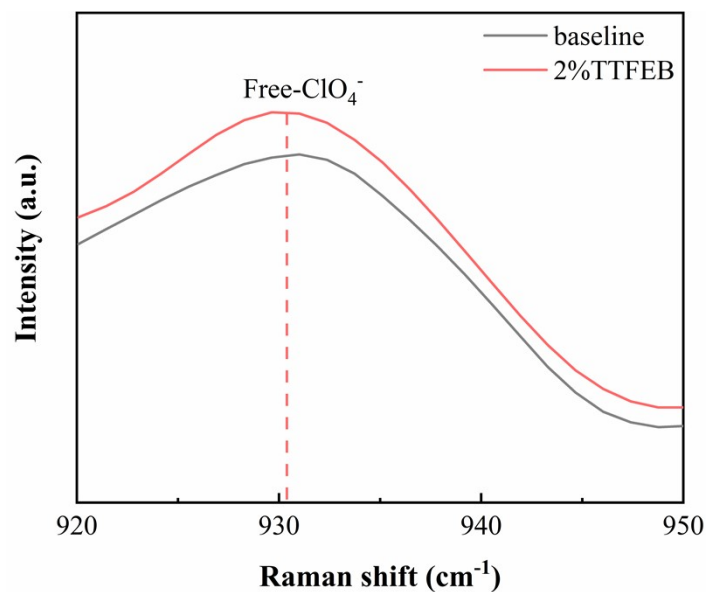
Fig. S1. The characteristic Raman spectra of \text{ClO}_4^- in different electrolytes.
