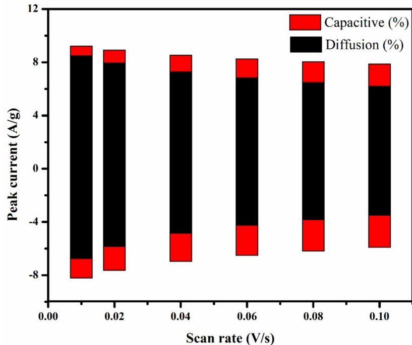
Figure S2: Contribution ratio of diffusion-controlled and capacitive-controlled processes of Fe-CoWO 4 electrode
