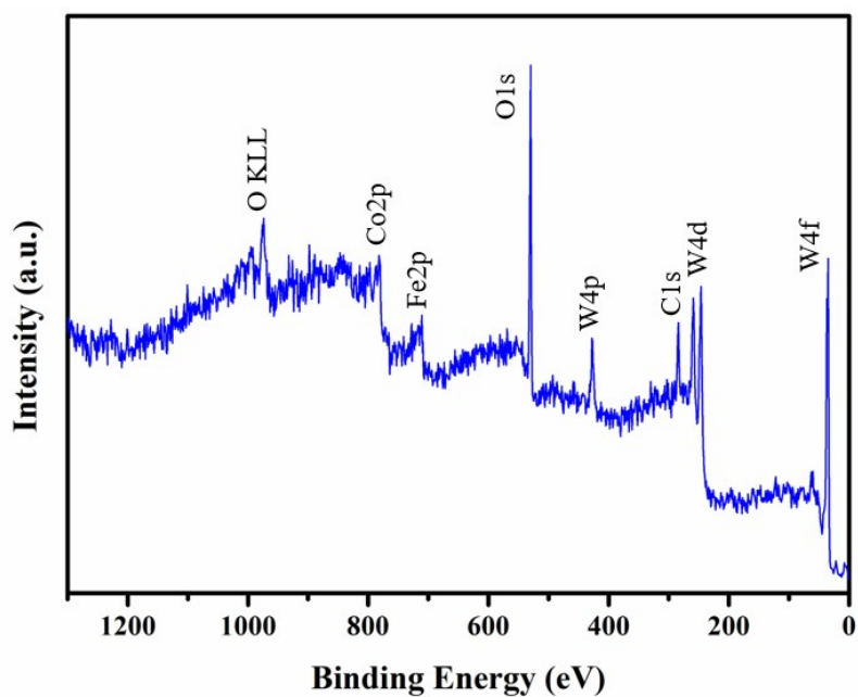
Figure S1: XPS survey spectrum of the prepared Fe-CoWO 4 sample
