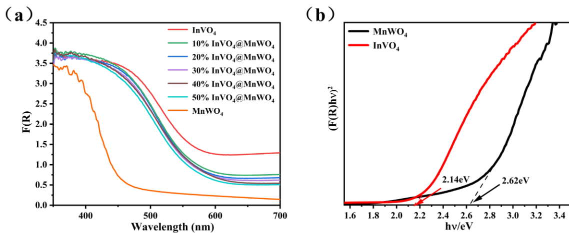
Fig. S5 (a) UV-vis DRS spectra of samples, (b) Tauc plots of \text{MnWO}_4 and \text{InVO}_4 .
