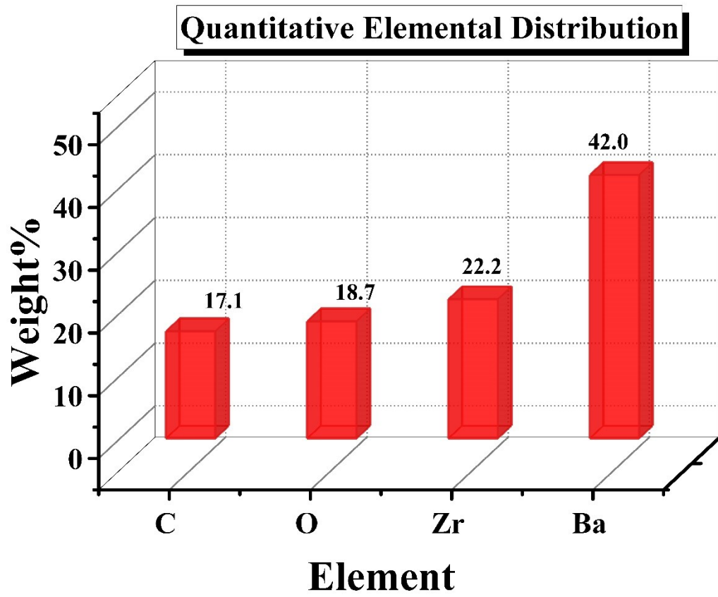
Figure S2. elemental distribution graph of BaZrO 3 nanoparticles.
