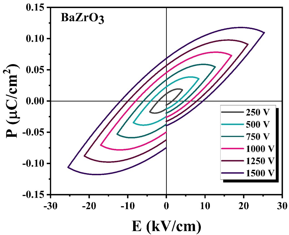
Figure S4. Ferroelectric PE Loop Analysis of BaZrO 3 ceramic.
