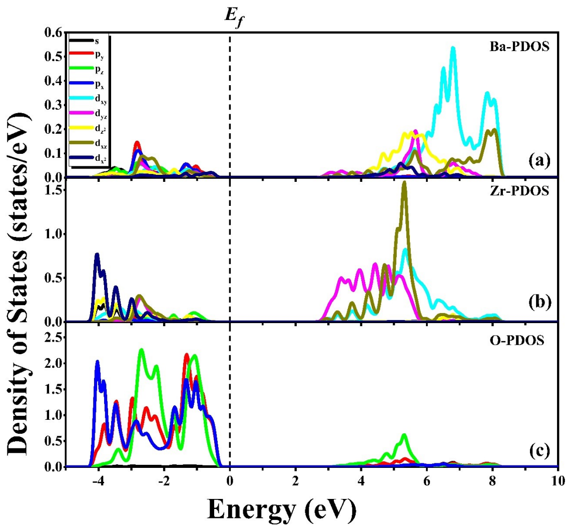
Figure S5. Partial Density of States (PDOS) of BaZrO 3 .
