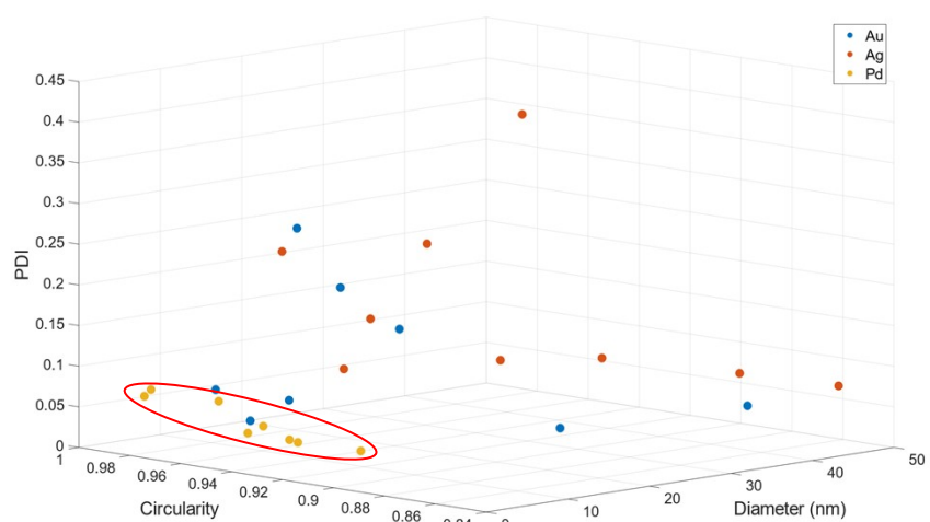
Figure S11. Tridimensional representation of all the responses spaces in respect to the metallic precursor (gold in blue, silver in red and palladium in yellow). Note the bias for the palladium experiments highlighted with a red circle, which displays similar diameters and PDIs, but varying circularities between the experiments.
