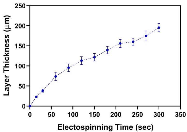
Figure S1. The duration of electrospinning linearly increases the coating thickness.
