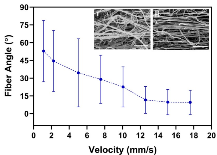
Figure S2. The angle of deposited electrospun fibers on the surface of the thread with increasing spooling speed. Inset images of (i) deposited fibers at 1 mm/s and (ii) 17 mm/s spooling velocities.
