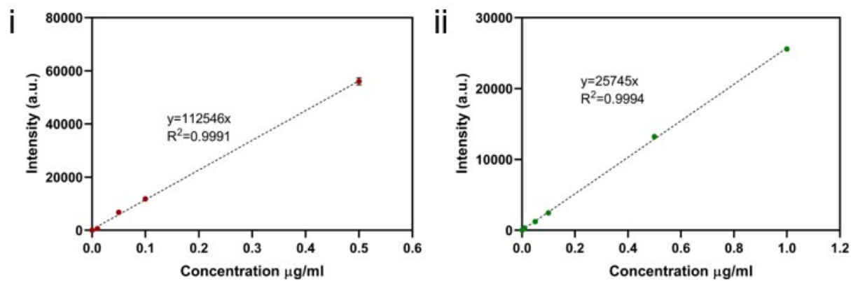
Figure S3. Experimentally determined calibration curves of fluorescence intensity for (i) Rhodamine B and (ii) FITC-Dextran in PECF.
