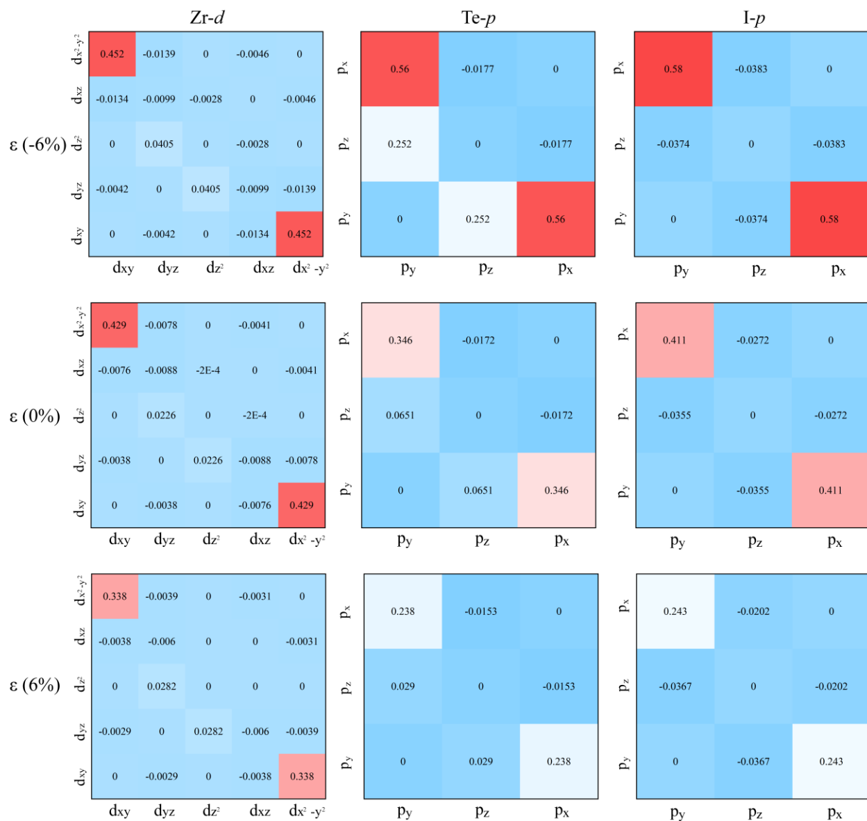
Fig. S9. Zr-d and Te/I-p orbital-resolved MAEs of Janus 2H-ZrTeI monolayers at 6%, 0% and 6% strain.
