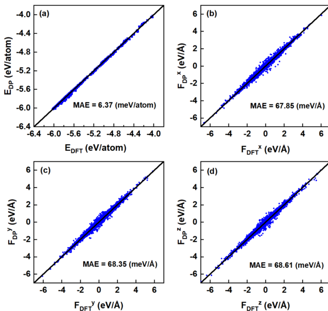
Fig. S1 Comparison of the results from the DP model and DFT calculations: (a) total energy of cluster, and forces on atom along the (b) x , (c) y , and (d) z directions.
