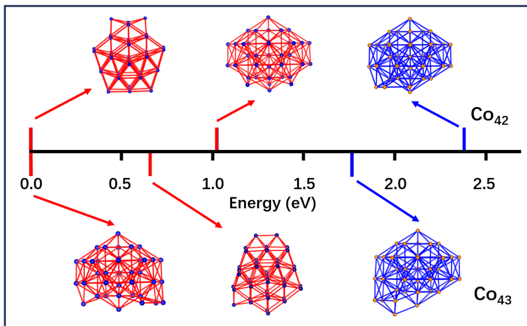
Fig. S2 Structures and relative energy distribution of \text{Co}_{42} and \text{Co}_{43} obtained by DP model. Colors indicate prediction comparisons: blue bonds represent structures already recorded in the CCD, while red bonds denote those newly identified using our DP model.
