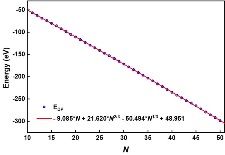
Fig. S4 The fitting curve of DP energy for \text{Co}_N ( N = 11\text{--}50 ) in our work.
