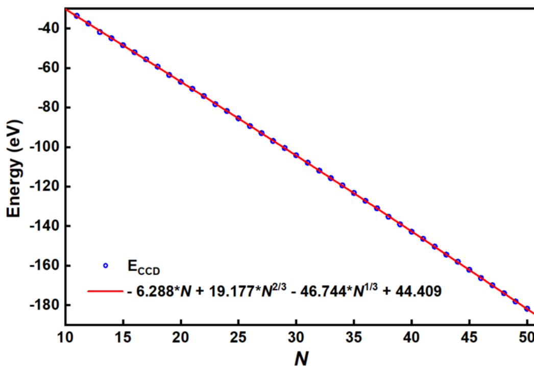
Fig. S3 The fitting curve of Gupta potential energy for \text{Co}_N ( N = 11-50 ) in CCD.
