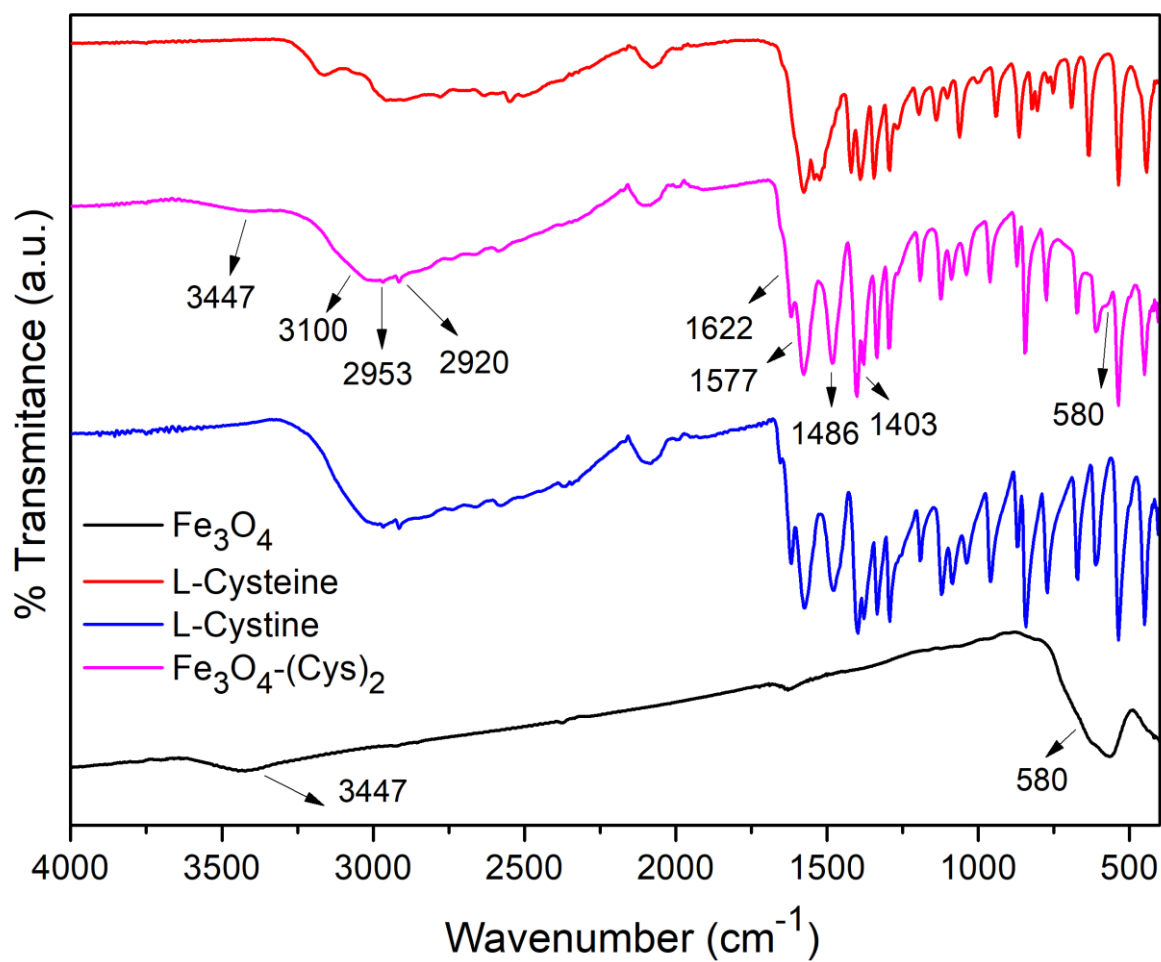
Figure S1: FTIR spectra of \text{Fe}_3\text{O}_4 nanoparticles (black line), L-Cysteine (red line), L-Cystine (blue line) and \text{Fe}_3\text{O}_4-(\text{Cys})_2 (magenta line)
