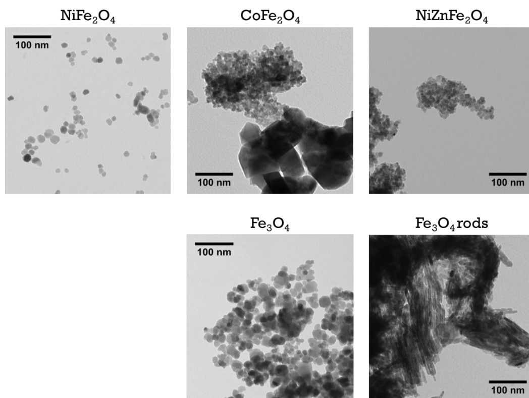
Figure S1: TEM images of the different magnetic nanoparticles.
